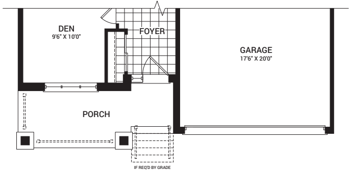
MAIN FLOOR PLAN C
