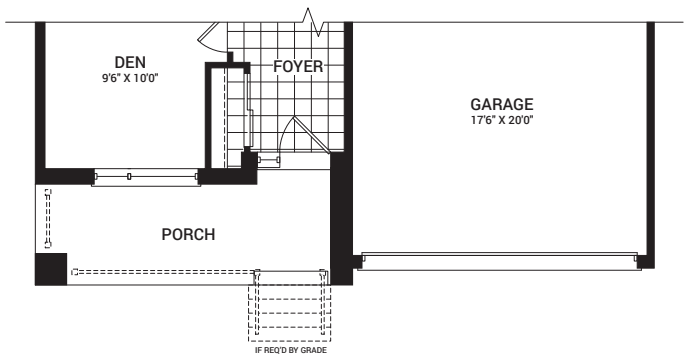
MAIN FLOOR PLAN D
